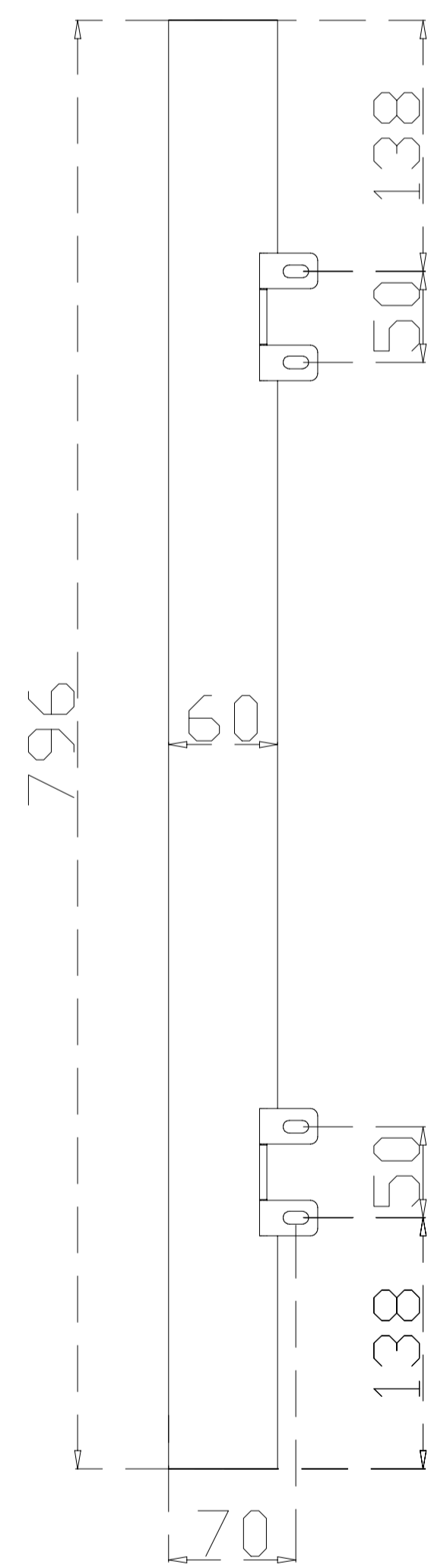
MQ 7608-K * 800 mm
